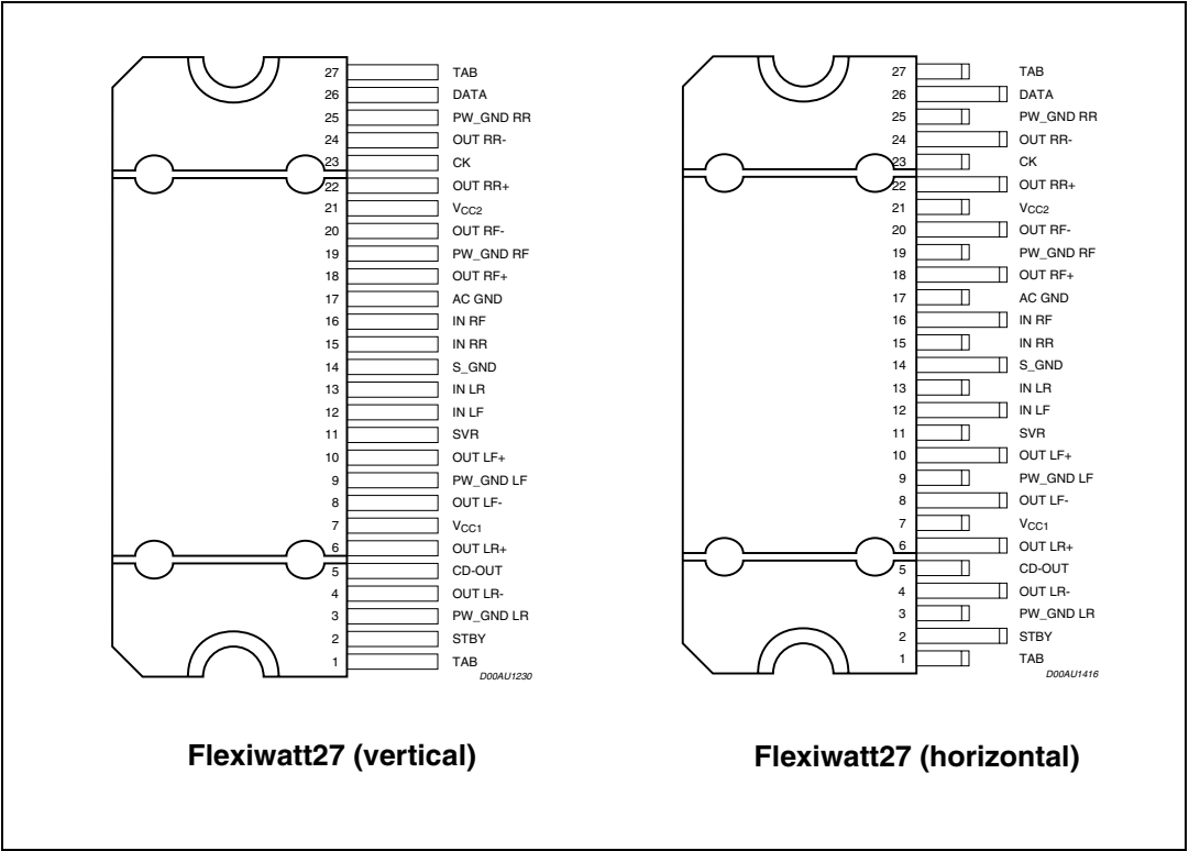
Figure 3. Pins connection diagram of the Flexiwatt27 (top of view)
